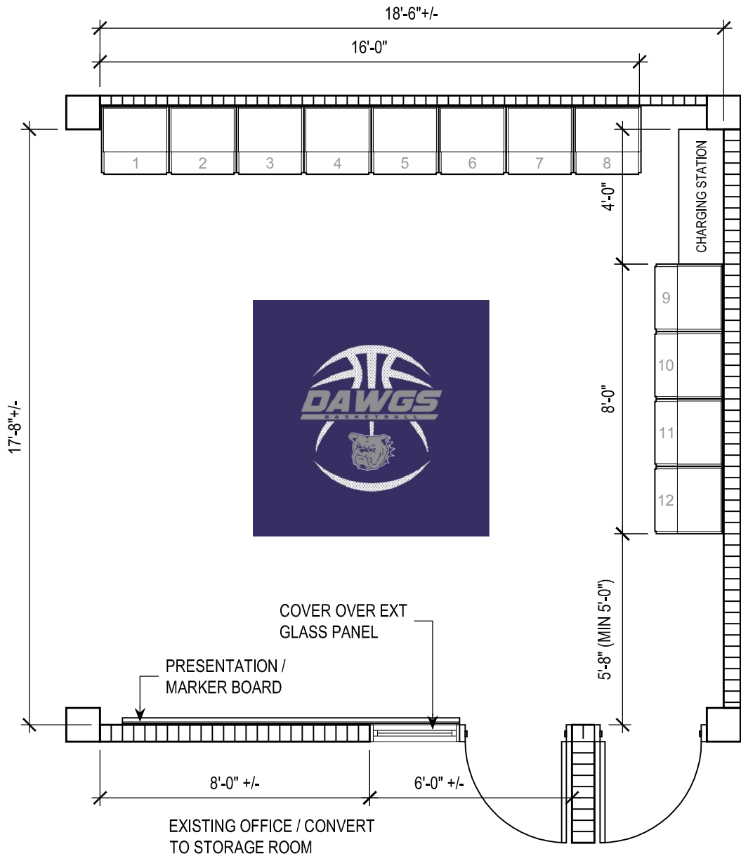
FIRST FLOOR PLAN 1
