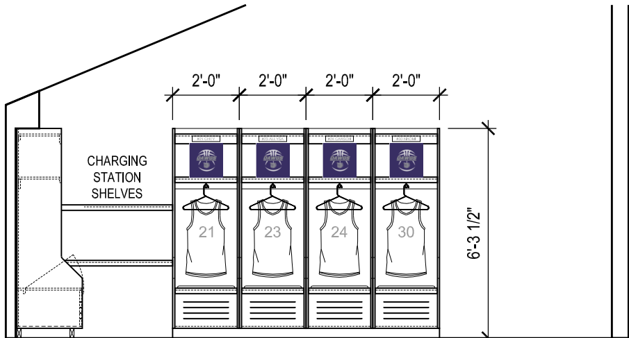
EAST ELEVATION
